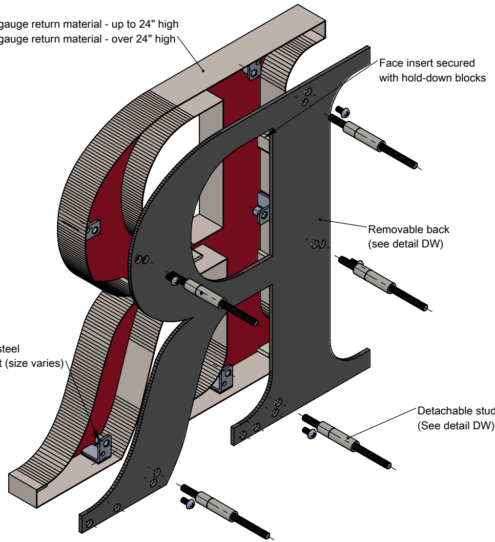
ISOMETRIC BACK VIEW II SCALE 1:3 BACK OPTIONS - Clear Lexan: 6-12" high - 0.118 thick - Light diffused plastic - Stainless steel - same gauge as face
