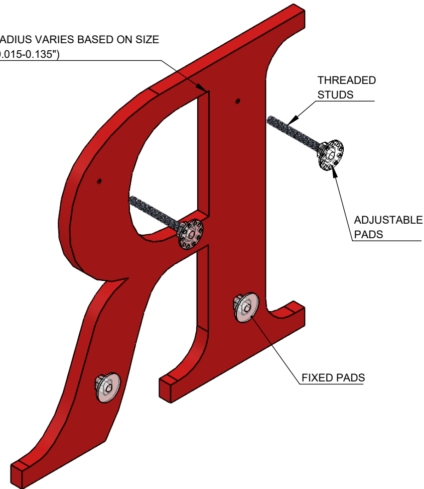
ISOMETRIC VIEW II SCALE 1:3
