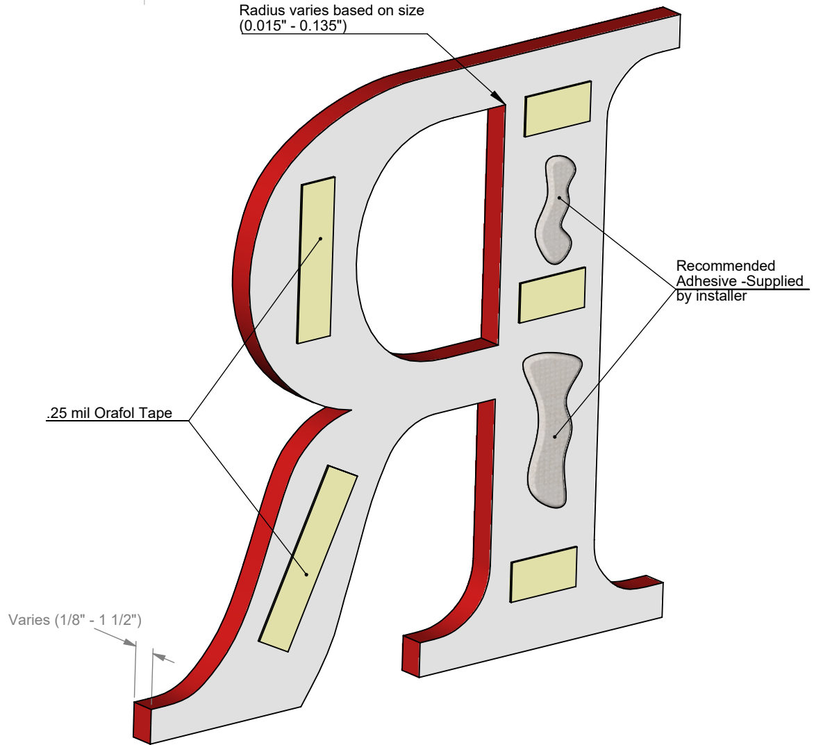
CUSTOM BACK VIEW II SCALE 1:3
