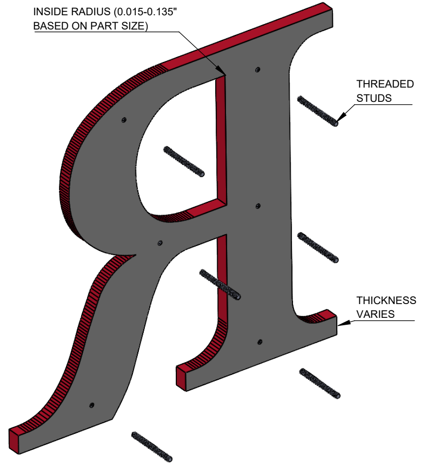
ISOMETRIC BACK VIEW II SCALE 1 : 3
