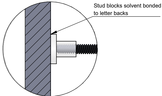
DETAIL DW SCALE 1 : 1
