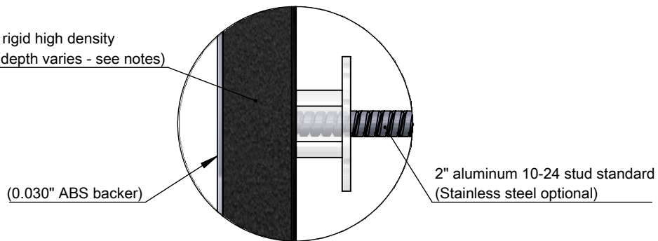
DETAIL DW SCALE 1 : 1
