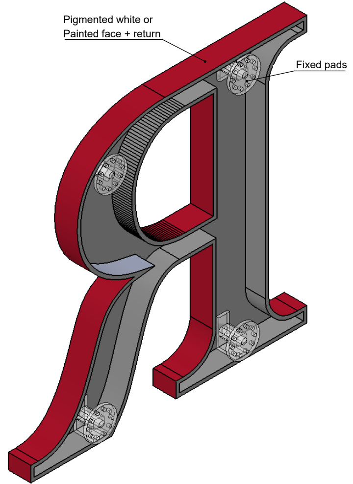
ISOMETRIC BACK VIEW II SCALE 1 : 3
