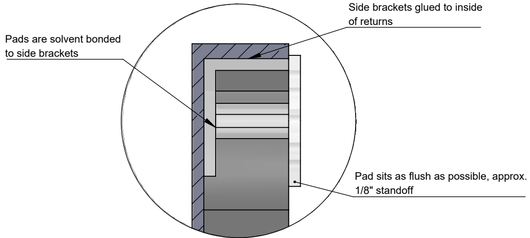
DETAIL DW II SCALE 1 : 1
