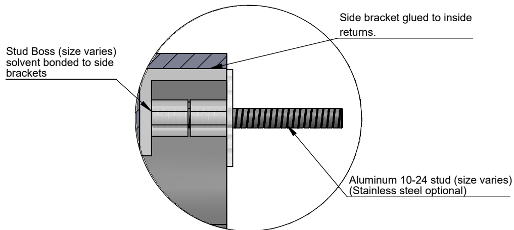
BACK VIEW II SCALE 1:5
