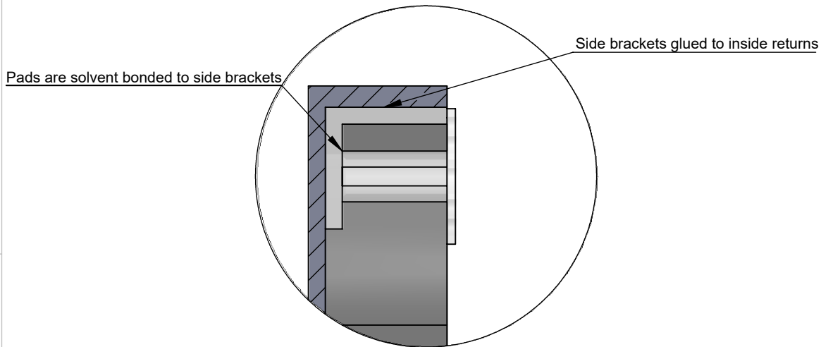
DETAIL DW II SCALE 1 : 1
